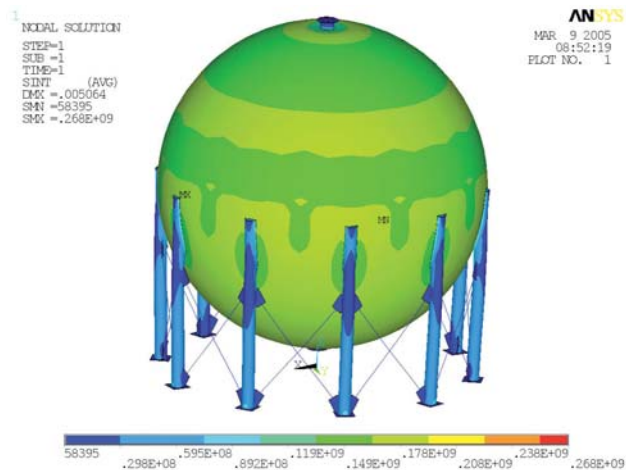
Finite element analysis of a spherical storage tank
